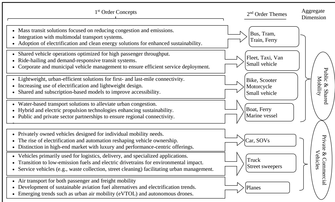
Fig. 2: Vehicle coding
