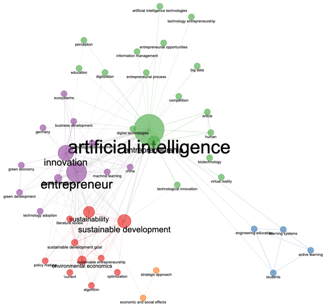
Fig. 6: Co-occurrence network
